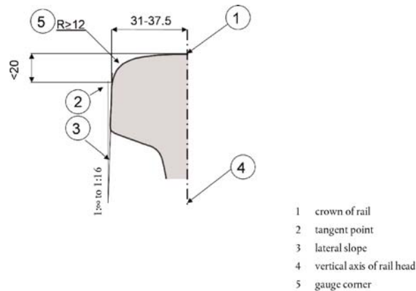
Railhead profile
