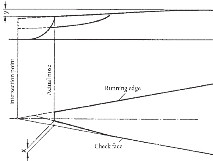
Figure 7 Point retraction X on check face
