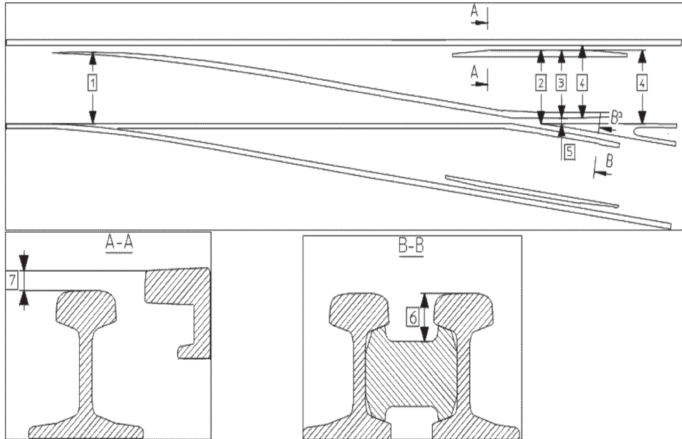
Figure 14 Geometry of switches and crossings
